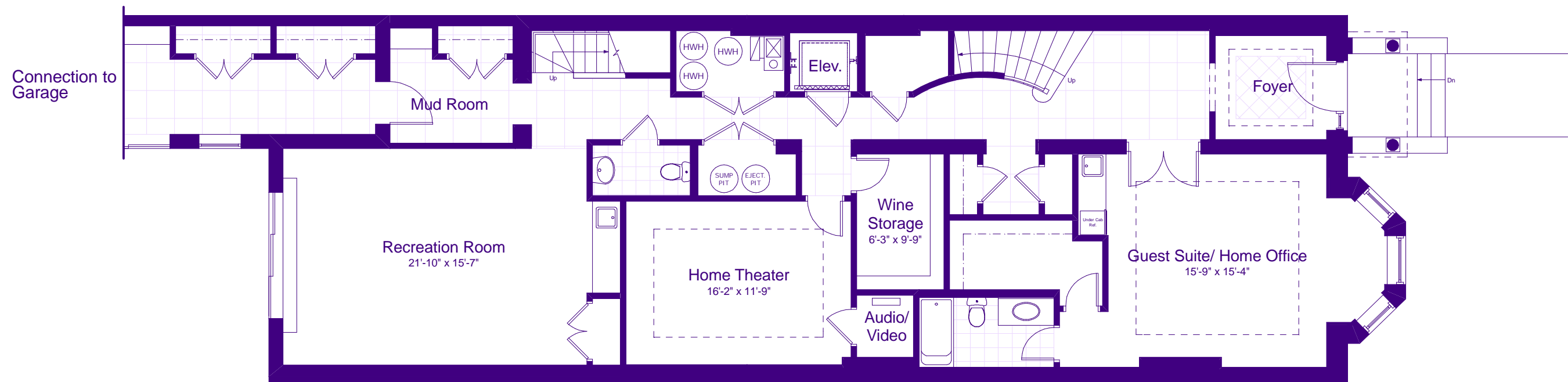
Alternate Ground Floor Plan
