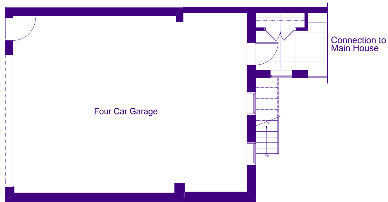
Alternate Garage Plan
